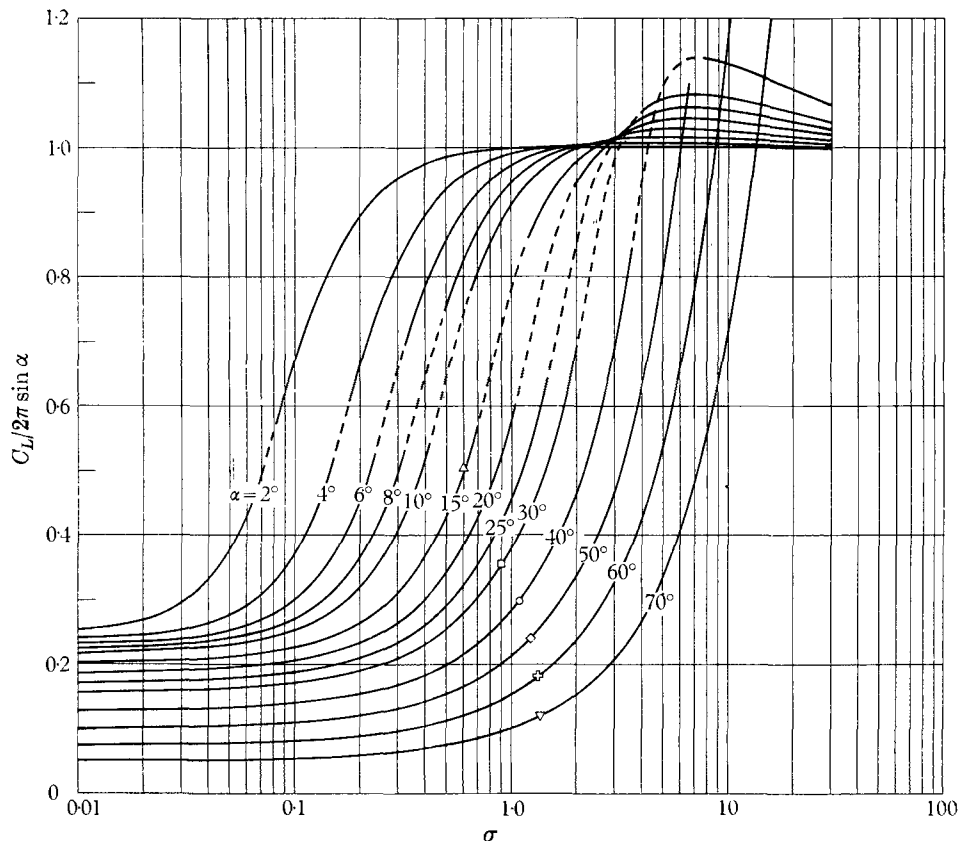
FIGURE 4. Variation of C_L over an extended range of \sigma to cover both the fully and partially developed wake flows past the flat plate, the transition between these two régimes of wake flows being appropriately faired-in with dashed lines. The experiments of Fage & Johansen were carried out in a wind tunnel, the results being reproduced with the wake under-pressure coefficient based on the measured constant base pressure and without the correction of the tunnel wall effect. —, Present theory. Fage & Johansen data: \Delta , \alpha = 15^\circ ; \square , \alpha = 30^\circ ; \circ , \alpha = 40^\circ ; \diamond , \alpha = 50^\circ ; \square with \times , \alpha = 60^\circ ; \nabla , \alpha = 70^\circ .
