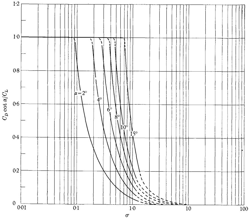
FIGURE 5. Variation of C_D over an extended range of \sigma for the flat plate. The dashed lines for \sigma > 1 are not the theoretical results, but are shown to indicate what would be expected on physical grounds.
